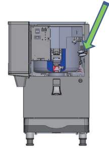
The area where the disinfectant and the sterilizing liquid is removed after the Agitator is removed.
