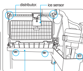
Water tank
